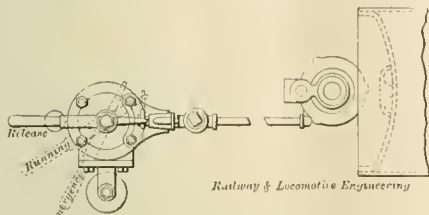
AUTOMATIC DRIVER BRAKE RETAINING VALVE.
